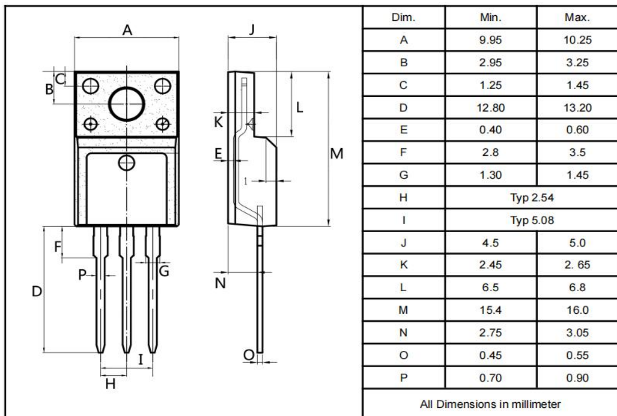
TO-220F
