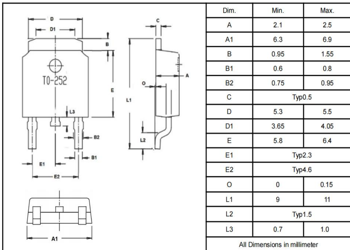
TO-252
